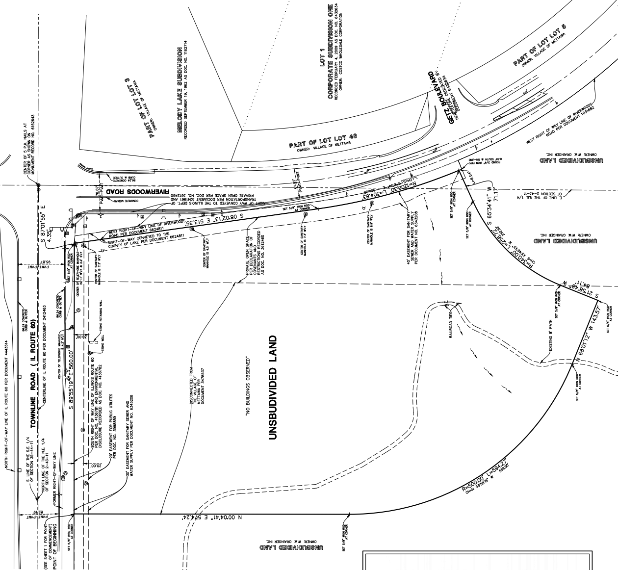
EASEMENT DETAIL "C" (DOC. NO. 3612460) NOT TO SCALE
